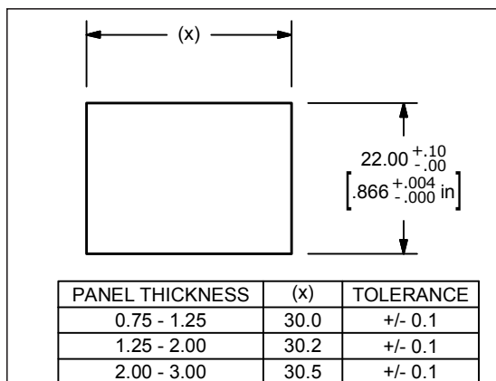
PANEL CUTOUT
