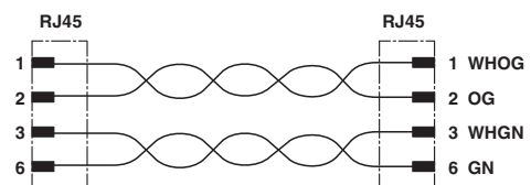
Circuit diagram
