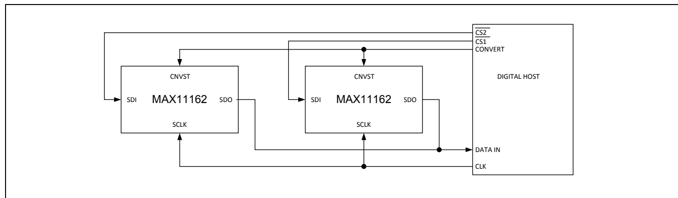
Figure 9. \overline{\text{CS}} Mode 4-Wire, No-Busy Indicator Connection Diagram
