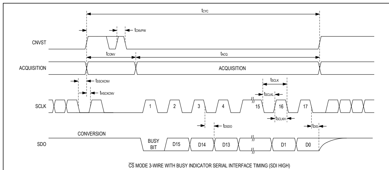
Figure 8. \overline{\text{CS}} Mode 3-Wire with Busy Indicator Serial Interface Timing (SDI High)
