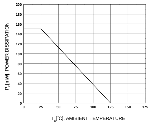
Figure 10. Power Derating
