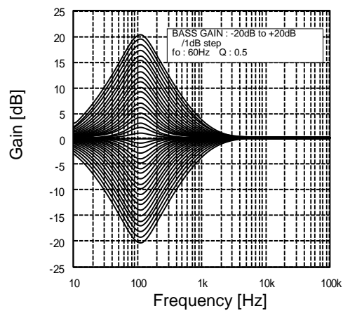
Figure 4. Bass Gain vs Frequency
