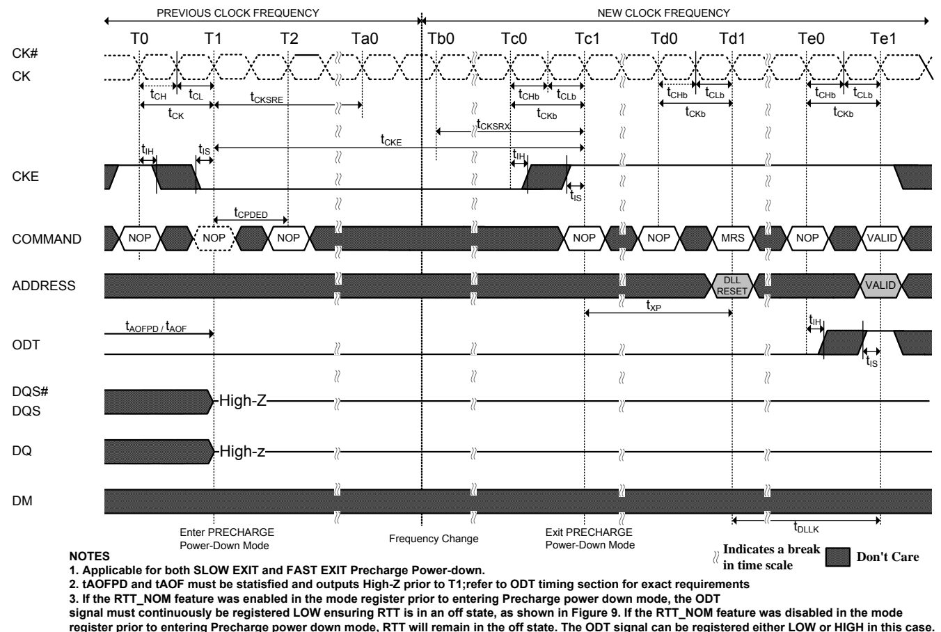
Figure 12. Change Frequency during Precharge Power-down
