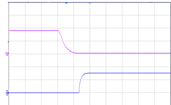
Figure 8 Output voltage startup by remote ON, (20ms/div), see Figure 11 for test configuration; CH1-output voltage (1V/div); CH2-remote ON voltage (2V/div) (Negative logic)
