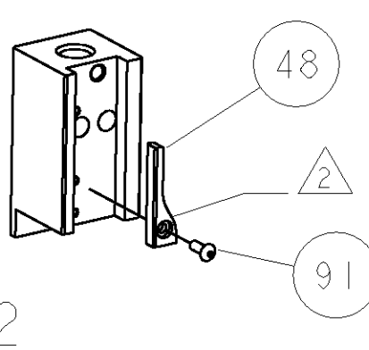
PRE-FEED 1 1/8 STROKE
