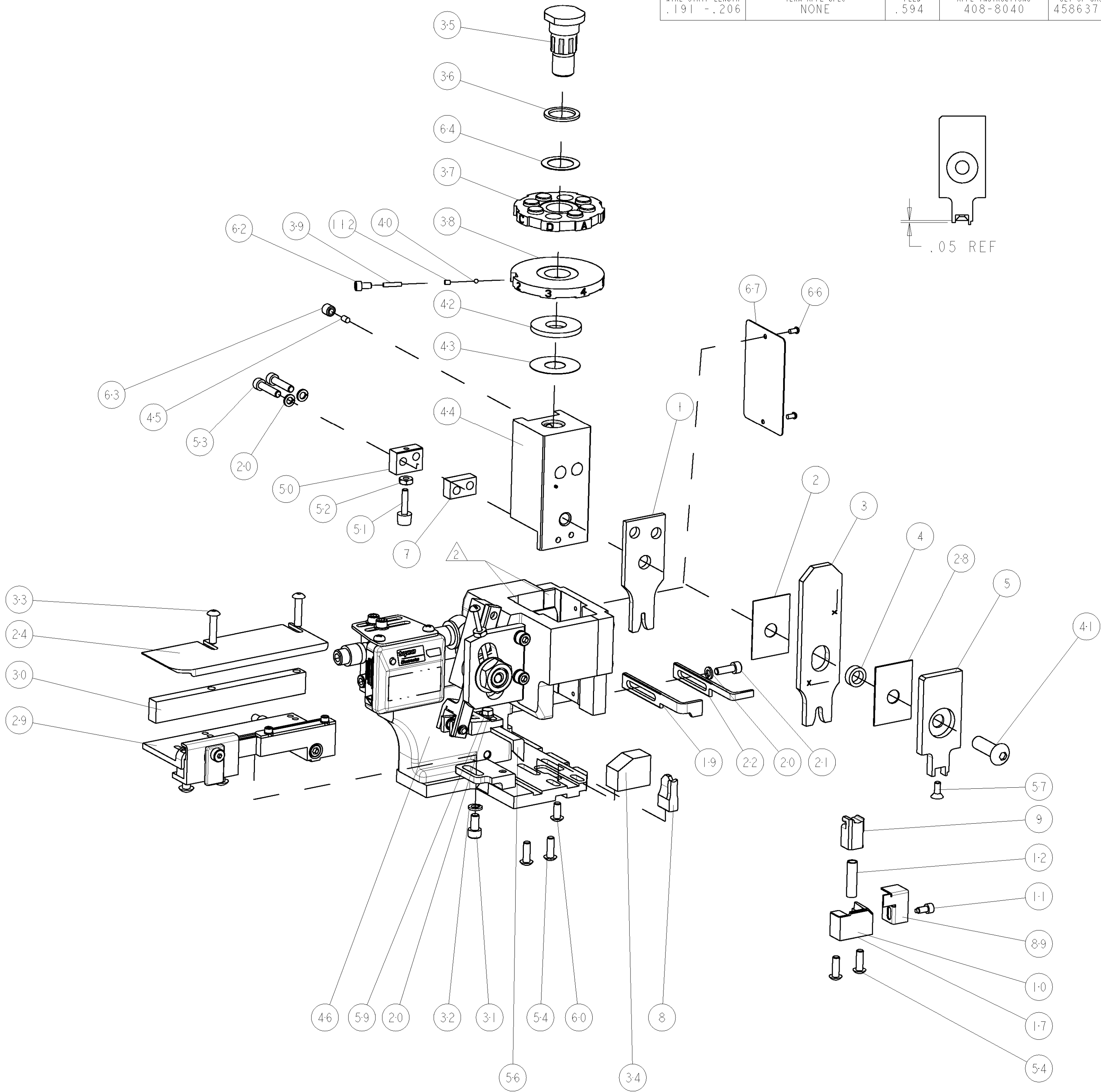
PRE-FEED 1 5/8 STROKE
