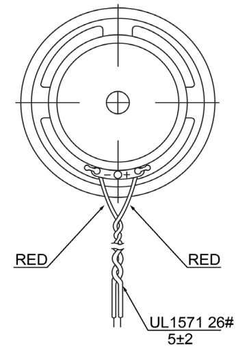
BOTTOM VIEW
