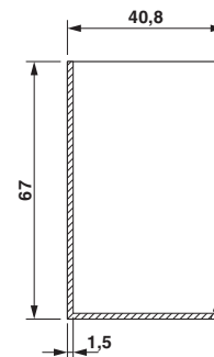
Dimensional drawing
