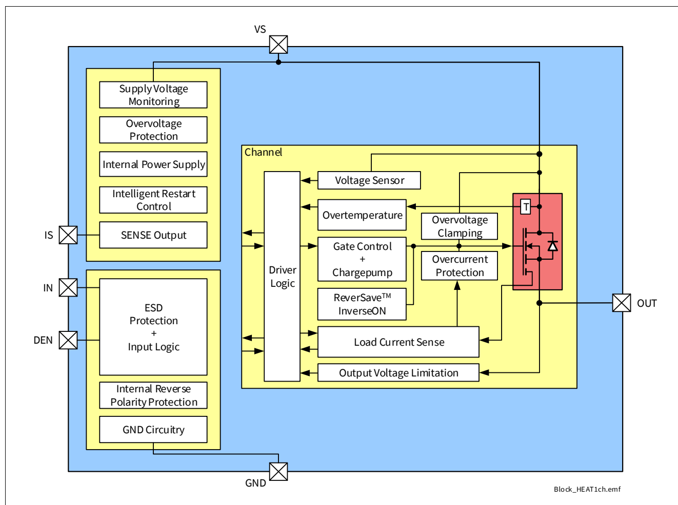
Figure 2 Block Diagram of BTS7004-1EPP
