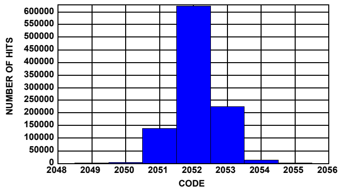
FIGURE 14. NOISE HISTOGRAM
