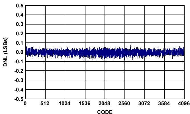
FIGURE 11. DIFFERENTIAL NONLINEARITY
