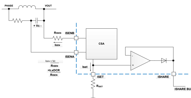
FIGURE 28. CURRENT SENSING BLOCK DIAGRAM
