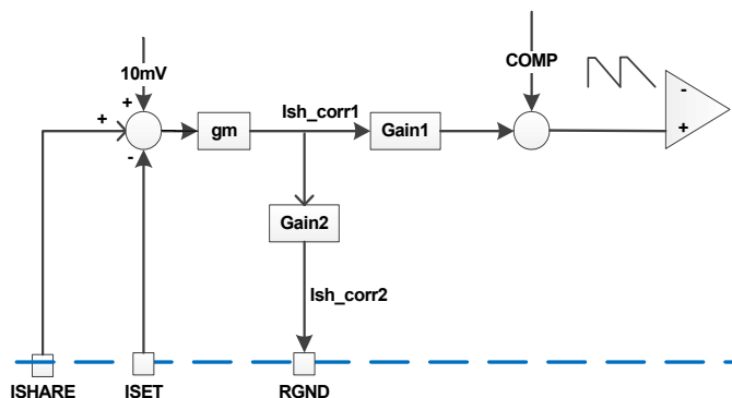
FIGURE 29. CURRENT SHARING BLOCK DIAGRAM
