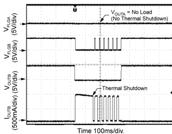
Independent Thermal Shutdown, Out B
