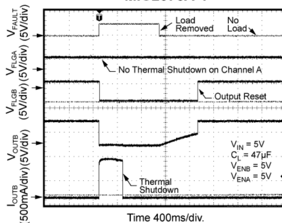
Independent Thermal Shutdown B MIC2076A-1
