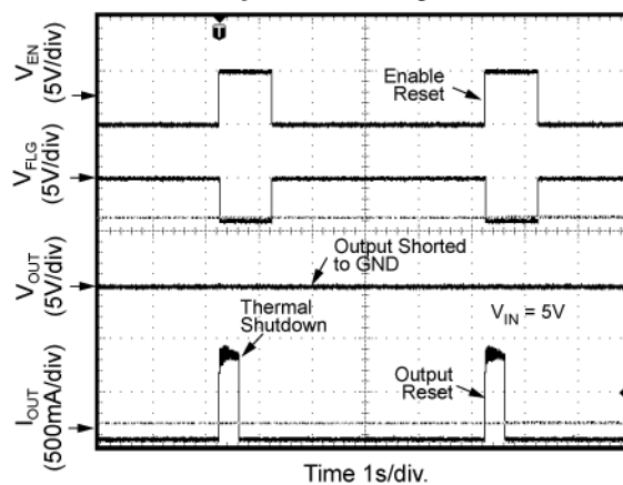
Thermal Shutdown MIC2076A-1: Output Reset by Enable
