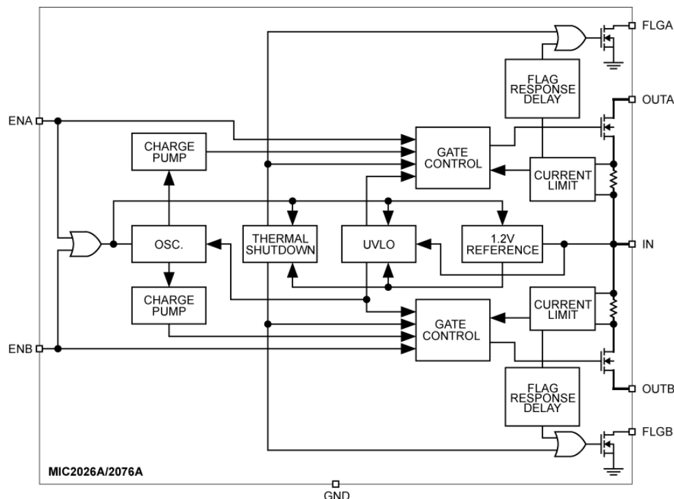
MIC2026A/2076A Block Diagram
