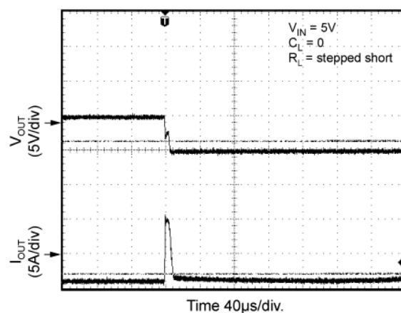
Current Limit Threshold, Zoom
