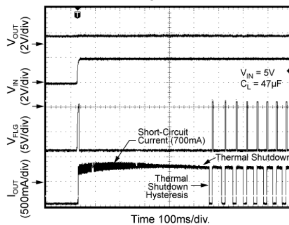
Current Limit Response, Output Short
