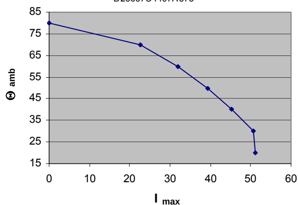
Max. allowable ambient Temp. at specific current (rms) B25667C4497A375
