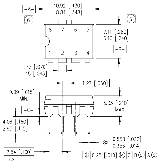
8 Lead PDIP
