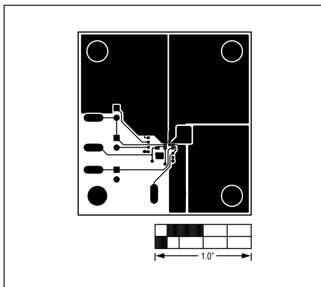
Figure 2. MAX15462A EV Kit PCB Layout—Component Side
