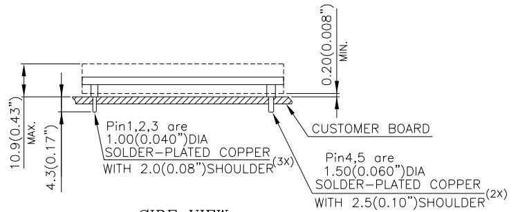
SIDE VIEW
