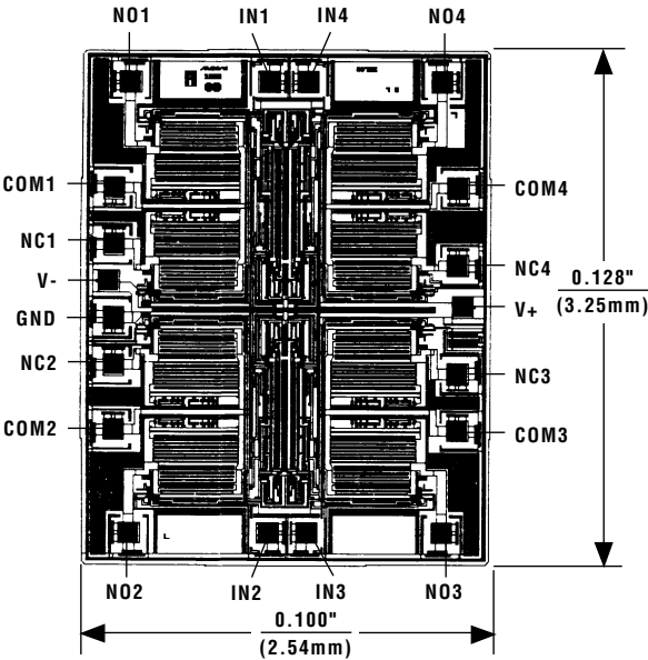
Chip Topography
