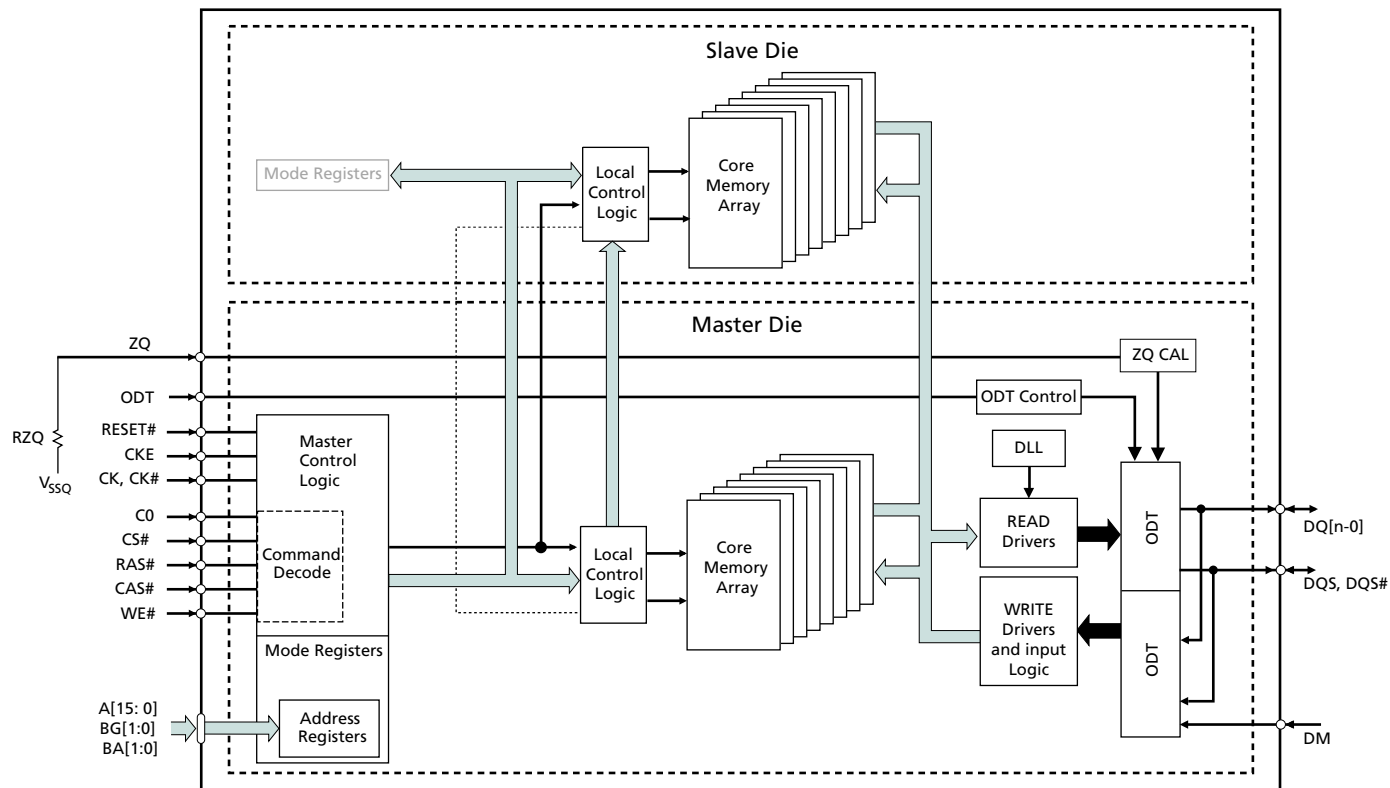
Figure 2: 2-high 3DS Device Functional Block Diagram
