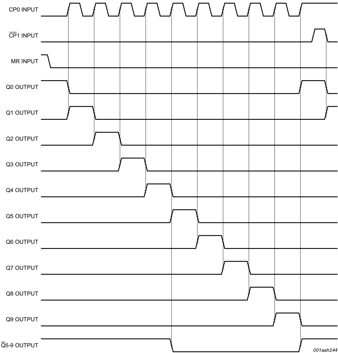
Fig 6. Timing diagram
