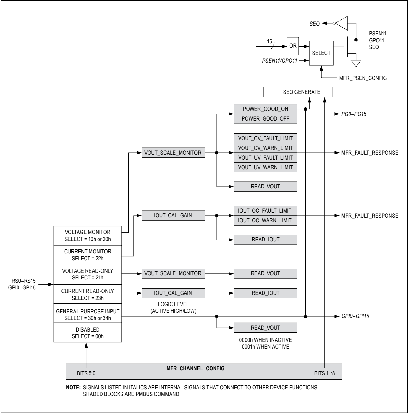
Figure 12. MFR_CHANNEL_CONFIG Command
