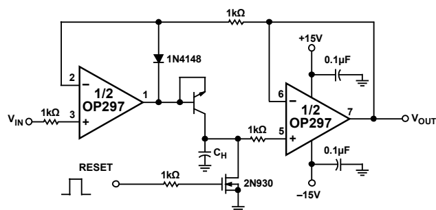
Figure 33. Precision Positive Peak Detector
