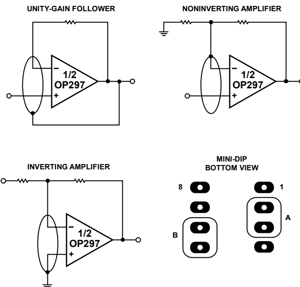
Figure 29. Guard Ring Layout and Considerations
