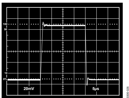
Figure 26. Small Signal Transient Response ( C_L = 100 pF, A_{VCL} = +1 )
