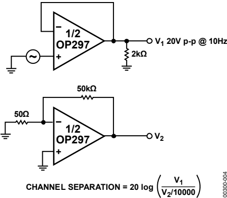
Figure 4. Channel Separation Test Circuit
