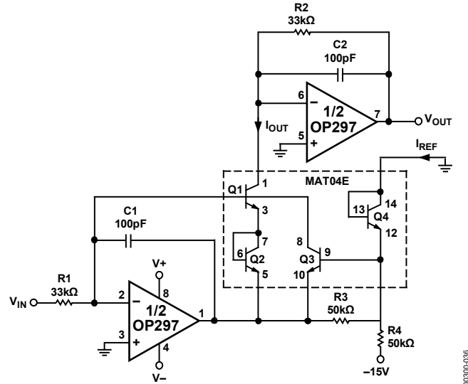
Figure 36. Square Root Amplifier
