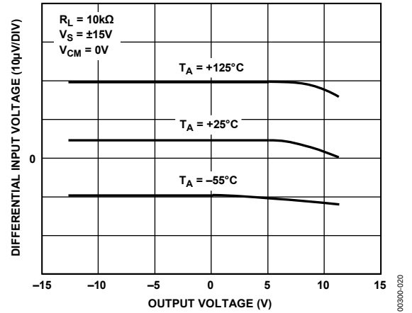
Figure 20. Differential Input Voltage vs. Output Voltage
