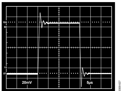
Figure 27. Small Signal Transient Response ( C_L = 1000 pF, A_{VCL} = +1 )
