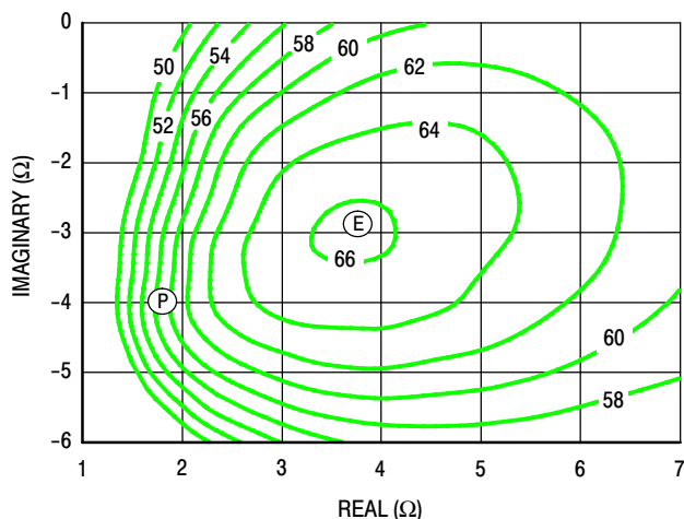
Figure 17. P3dB Load Pull Efficiency Contours (%)
