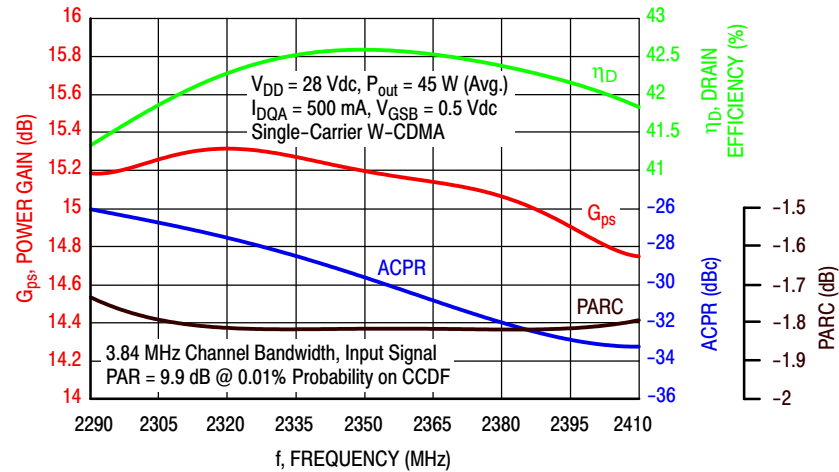
Figure 3. Single-Carrier Output Peak-to-Average Ratio Compression (PARC) Broadband Performance @ P_{out} = 45 Watts Avg.
