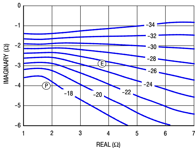
Figure 19. P3dB Load Pull AM/PM Contours (°)
