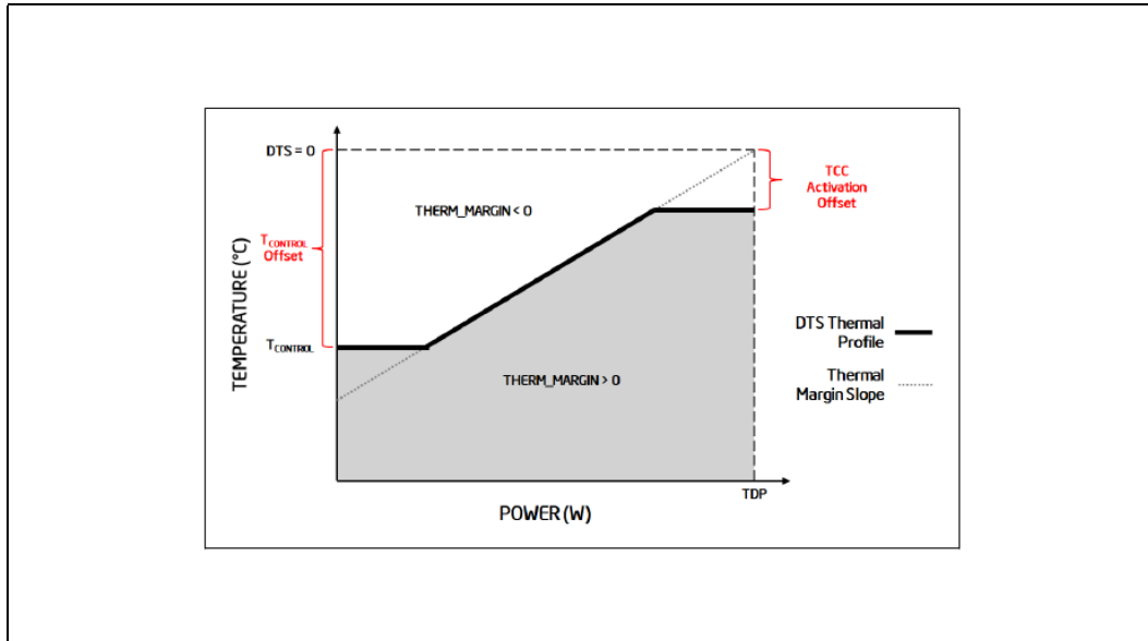
Figure 5-3. Digital Thermal Sensor (DTS) 2.0 Definition Points
