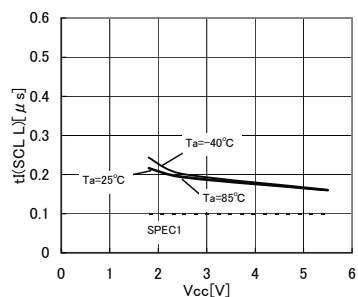
Fig.30 Noise removal valid time t_I(\text{SCL L})
