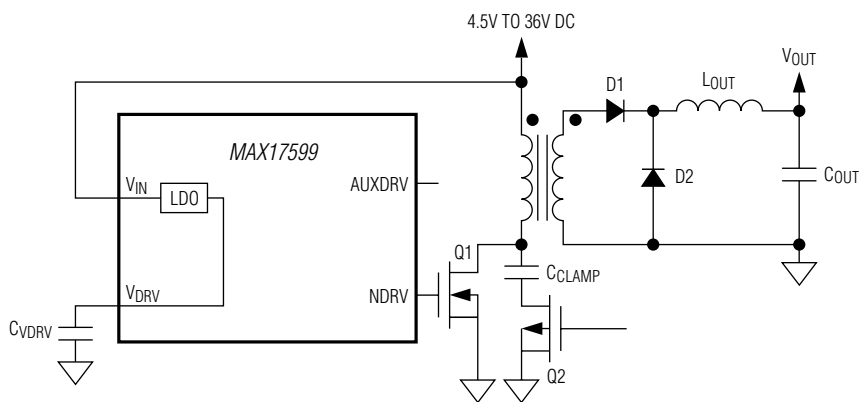
Figure 4. Typical Startup Circuit with IN Connected Directly to DC Input
