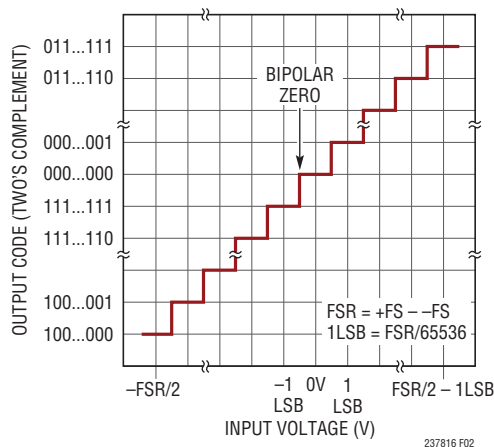
Figure 2. LTC2378-16 Transfer Function
