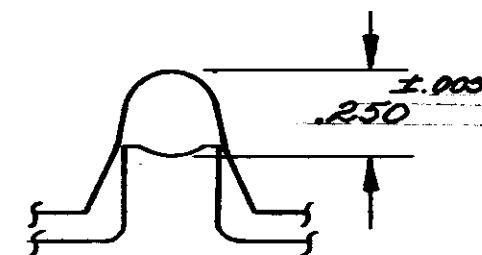
DIE-INSULATION CRIMP
