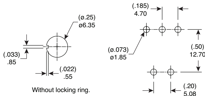
Panel Mounting
