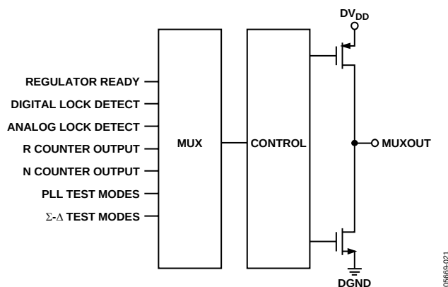
Figure 21. MUXOUT Circuit
