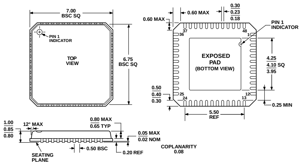
Figure 57. 48-Lead Lead Frame Chip Scale Package [LFCSP_VQ]
