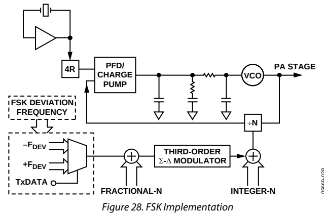
Figure 28. FSK Implementation
