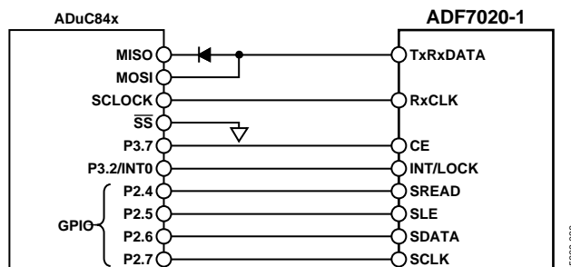
Figure 36. ADuC84x to ADF7020-1 Connection Diagram
