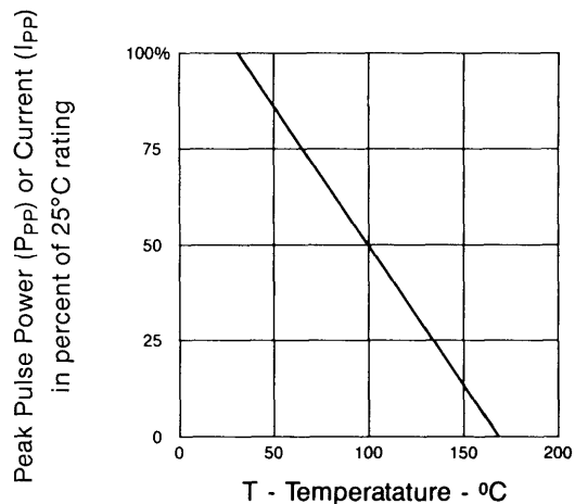
FIGURE 2 DERATING CURVE
