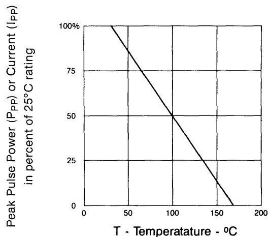
FIGURE 2 DERATING CURVE
