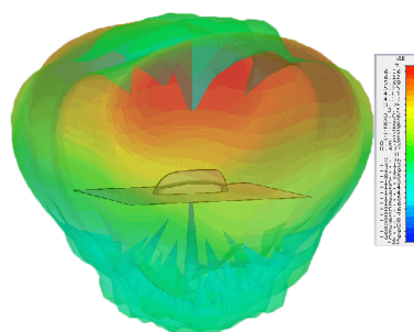
3D Gain Plot Top (3600MHz)
