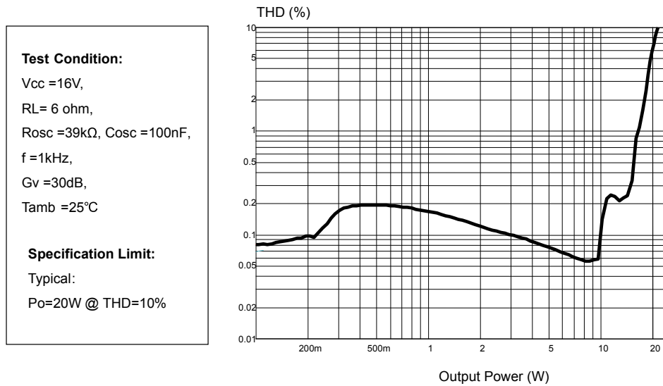
Figure 20. THD vs. output power (1 kHz)
