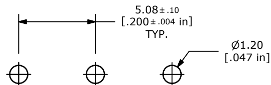
P.C. MOUNTING
