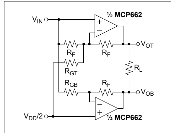
FIGURE 4-12: H-Bridge Driver.
