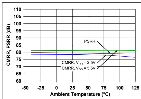
FIGURE 2-9: CMRR and PSRR vs. Ambient Temperature.
