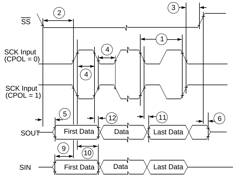
Figure 26. DSPI Classic SPI Timing — Slave, CPHA = 0
