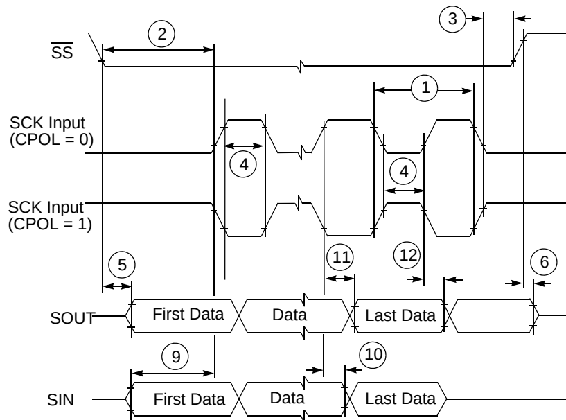
Figure 30. DSPI Modified Transfer Format Timing — Slave, CPHA = 0
