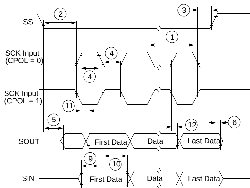
Figure 27. DSPI Classic SPI Timing — Slave, CPHA = 1
