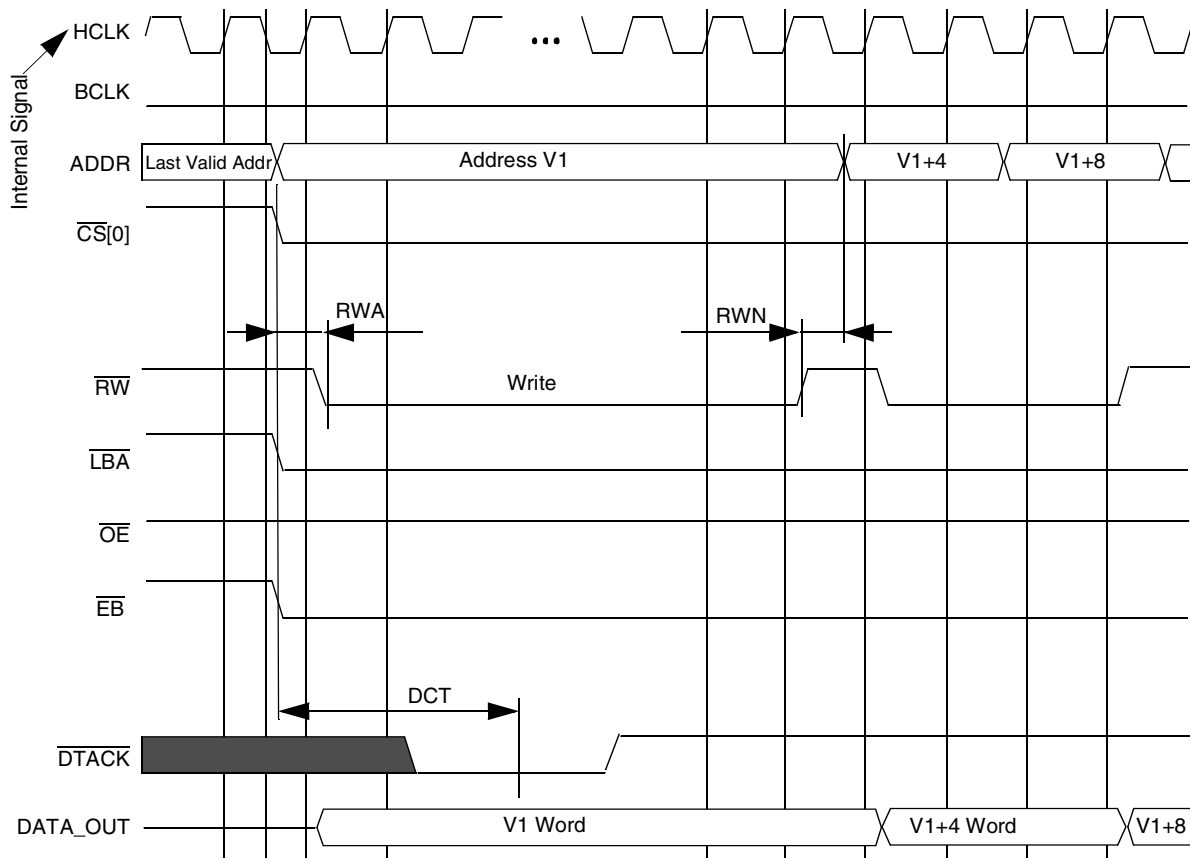
Figure 71. DTACK Level Sensitive Sequential Write Accesses, WSC=2, EW=1, RWA=1, RWN=1, DCT=1, AGE=0 (Example of \overline{DTACK} Asserting)
