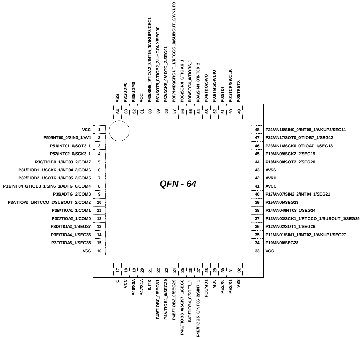
(TOP VIEW)
