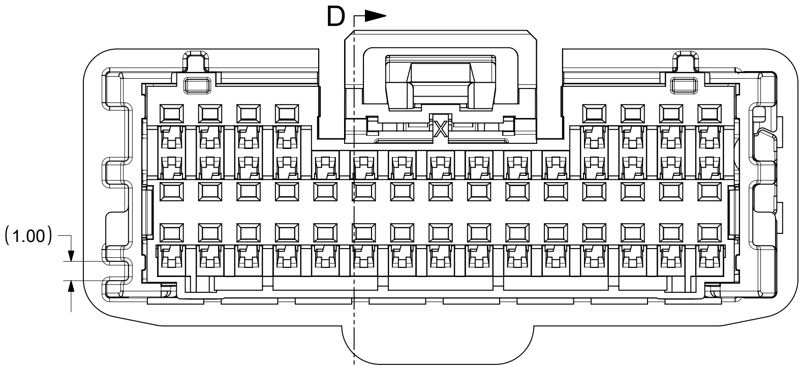
38 WAY UPDATED POLARIZATION P/N: 34959-038X(X=3, 4, 5) 34959-039X(X=0, 1, 2)
