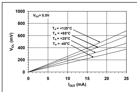
FIGURE 2-24: Output Headroom Vs Output Current.
