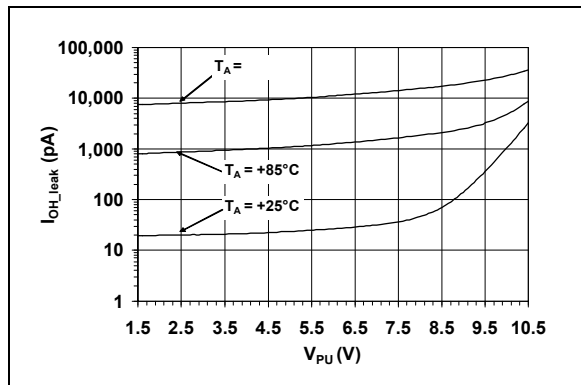
FIGURE 2-23: Output Leakage Current vs. Pull-up Voltage.
