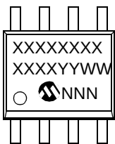
8-Lead SOIC (150 mil) (MCP6567)
