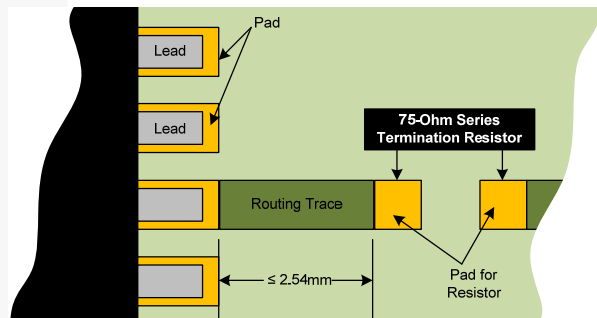
Figure 13. Termination Resistor
