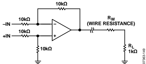
Figure 51. Wire Resistance Causes Errors at Load Voltage
