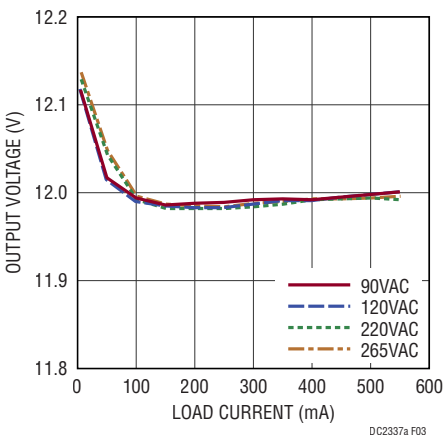
Figure 3. Load and Line Regulation
